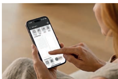
HomeComfort App
